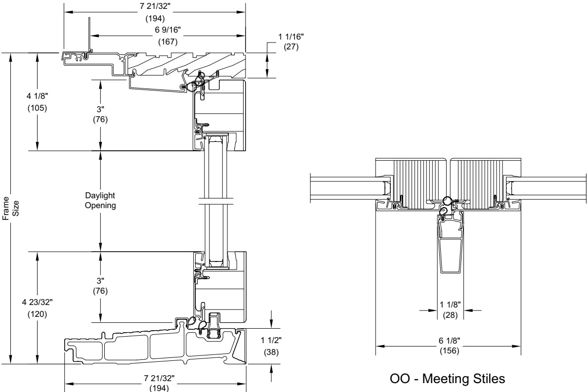
6 9/16" Head Jamb and Sill
