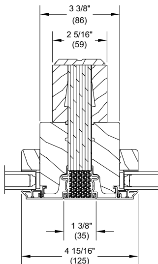
1" LVL Mullion
