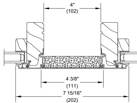
4" Space Mull
