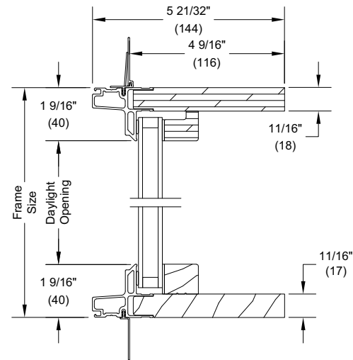
Head Jamb and Sill
