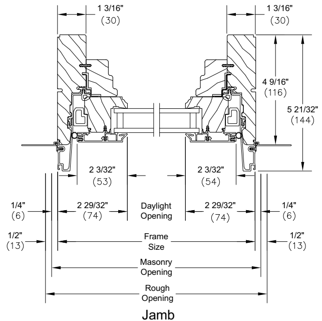
Stationary/Picture - 1" IG
