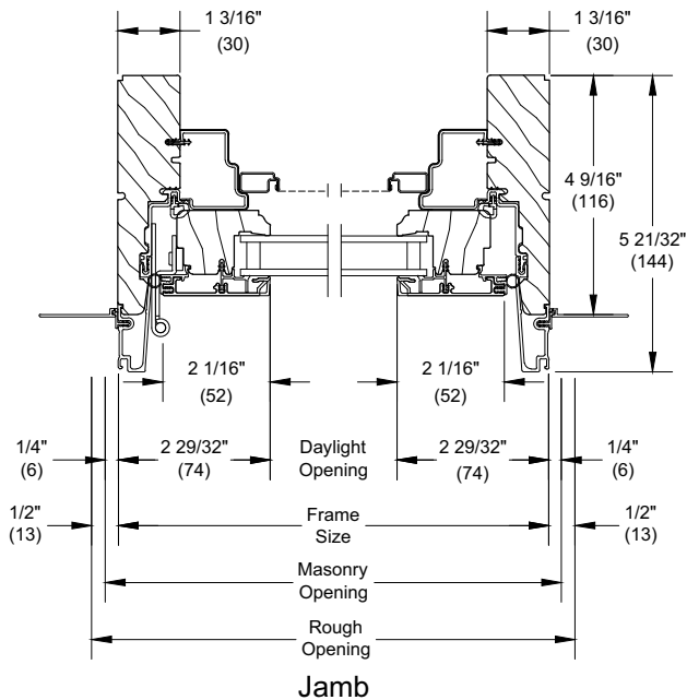
Operating - 3/4" IG
