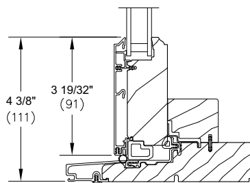
Wide Bottom Rail Option Stationary (3/4" IG)
