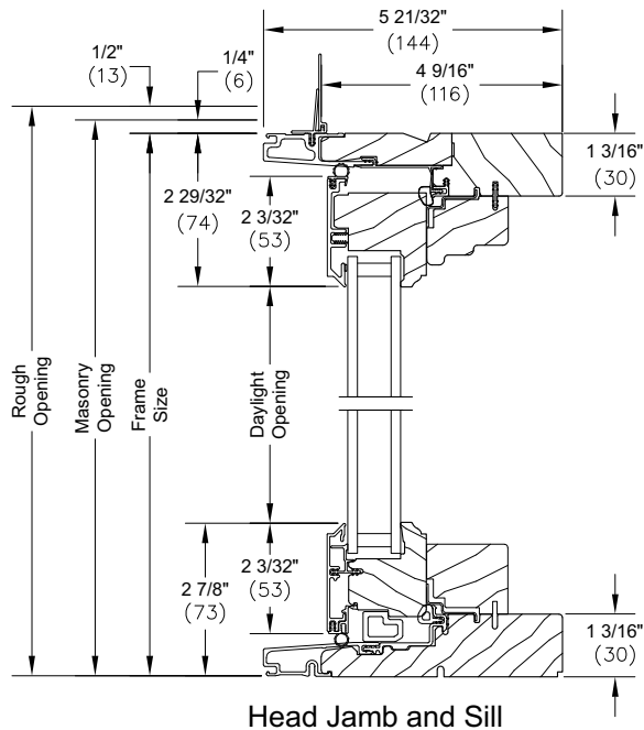
Stationary/Picture - 1" IG
