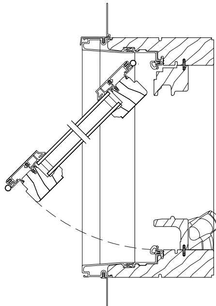
Vent Opening
