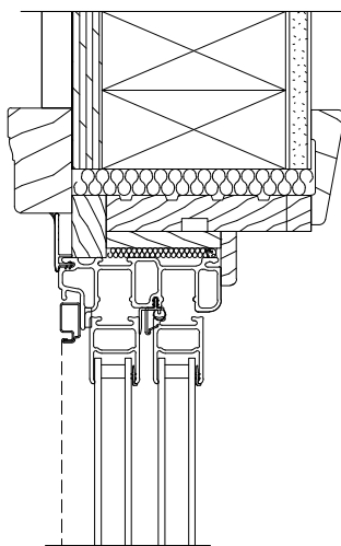
Head Jamb Frame Expander
