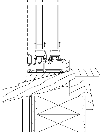
Sill Frame Expander
