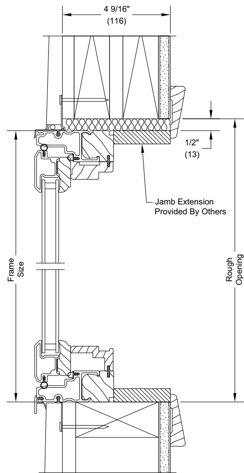
Head Jamb and Sill Nailing Fin Install
