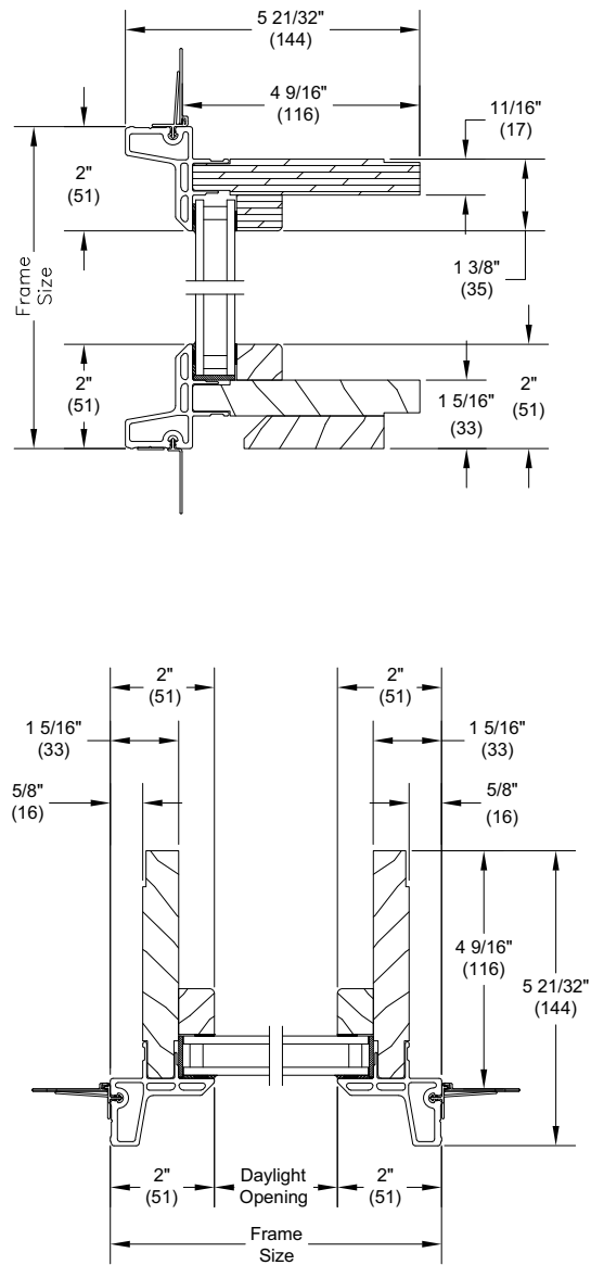
CASEMENT - 4 9/16"
