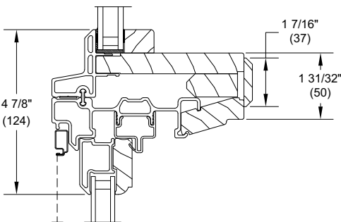
Round Top Over Double Hung
