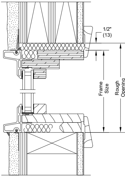
Stucco With 2X4 Frame Construction
