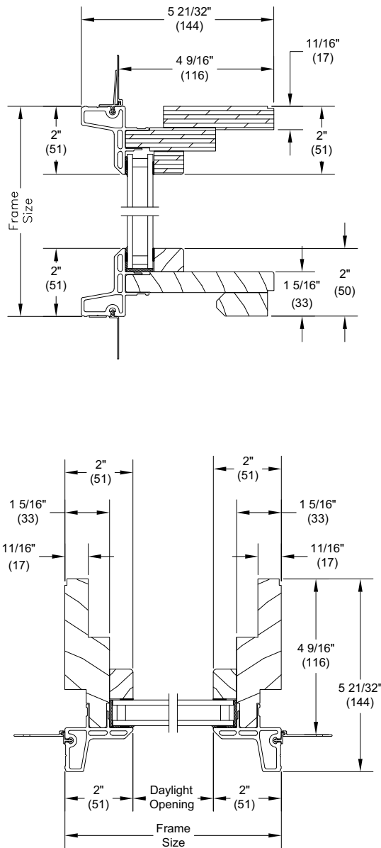
DOUBLE HUNG/DOOR - 4 9/16"
