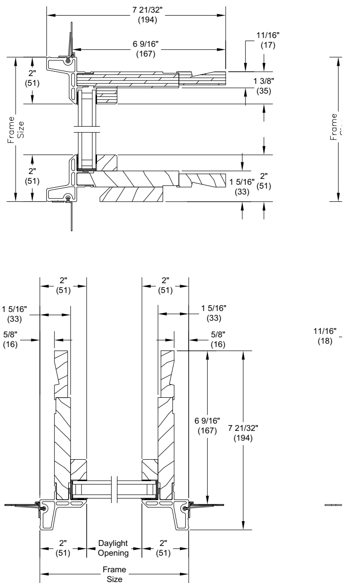
CASEMENT - 6 9/16"
