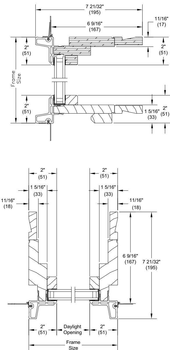
DOUBLE HUNG/DOOR - 6 9/16"
