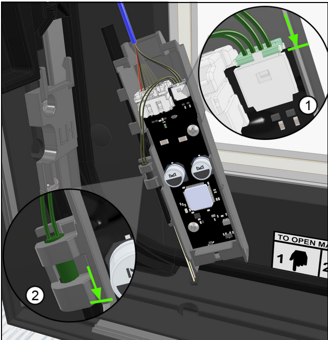
Figure 31 MCB Connections
