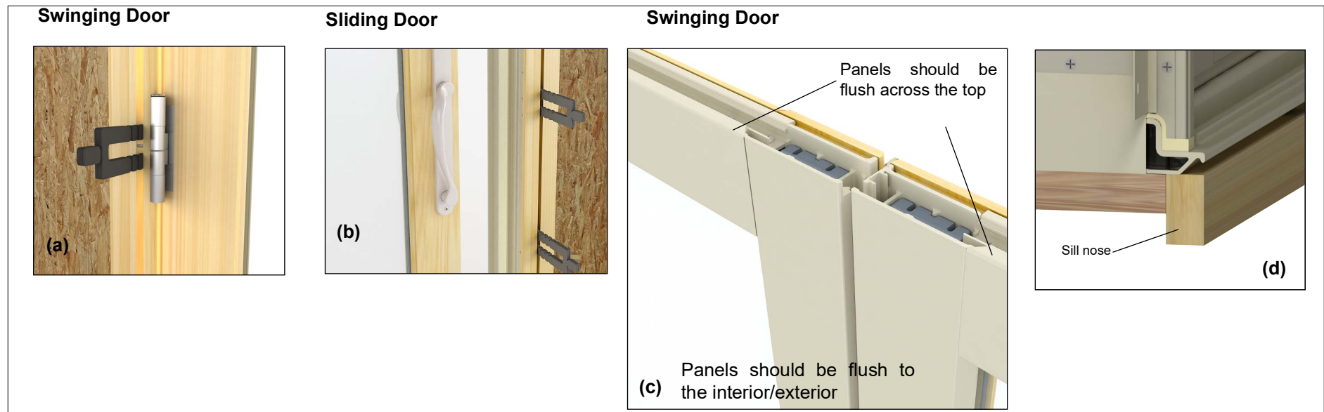
Figure 5 Shimming the door
