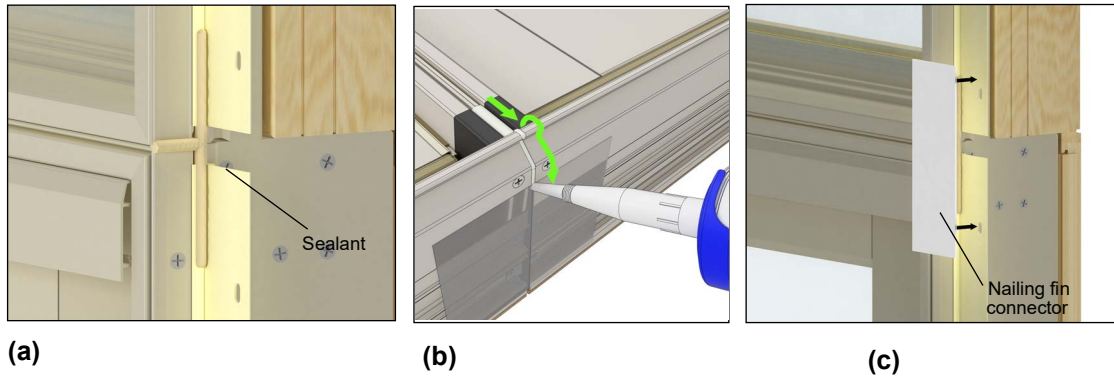
Figure 3 Preparing the unit for installation.
