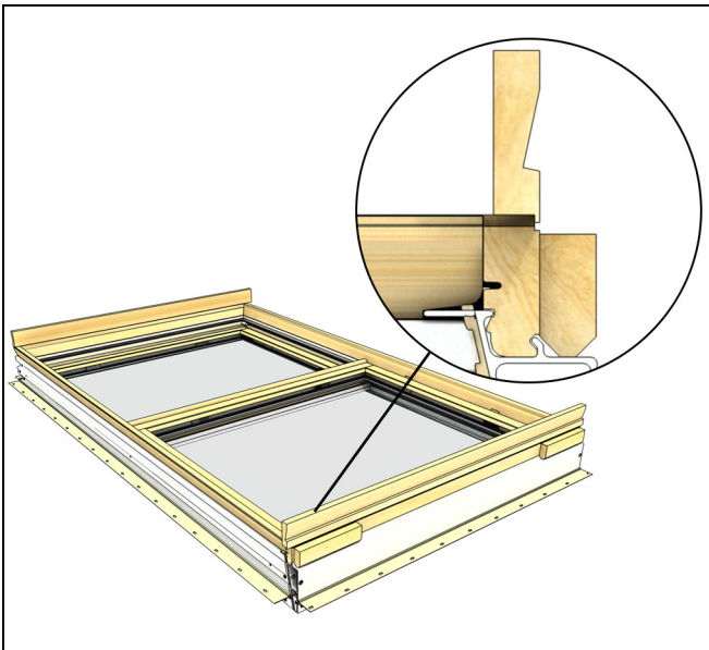
Figure 1 Fastener spacing see fastener table
