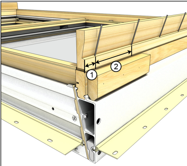
Figure 1 Fastener spacing see fastener table
